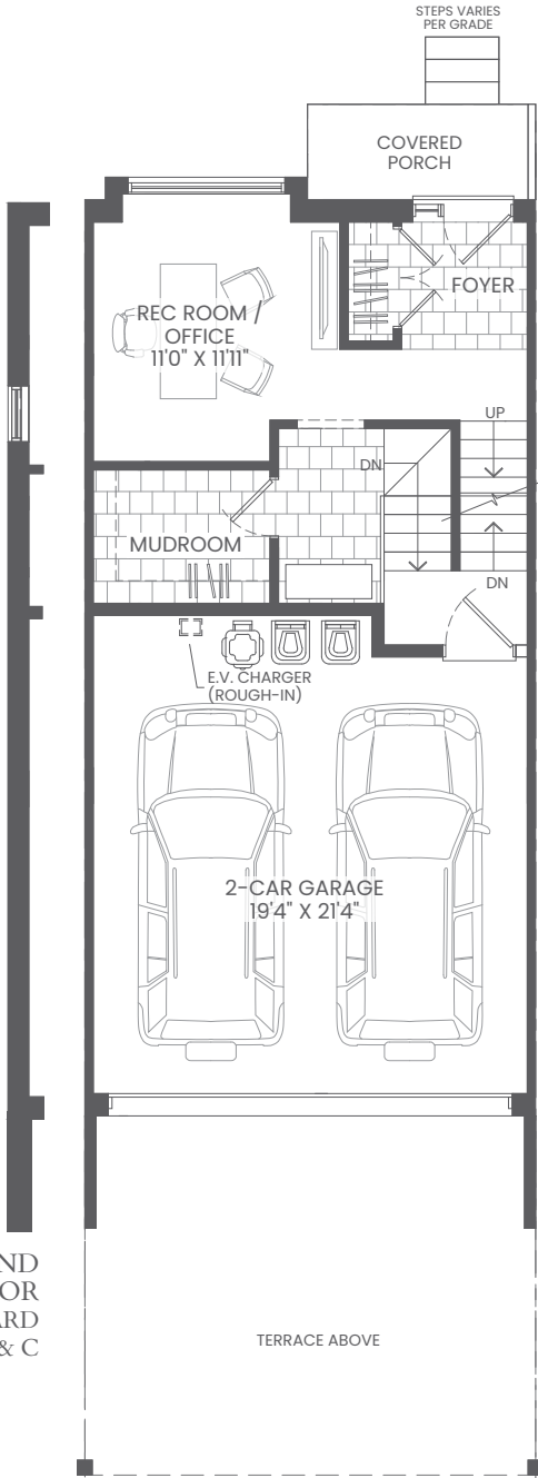
GROUND FLOOR STANDARD INTERIOR BLK B & C
