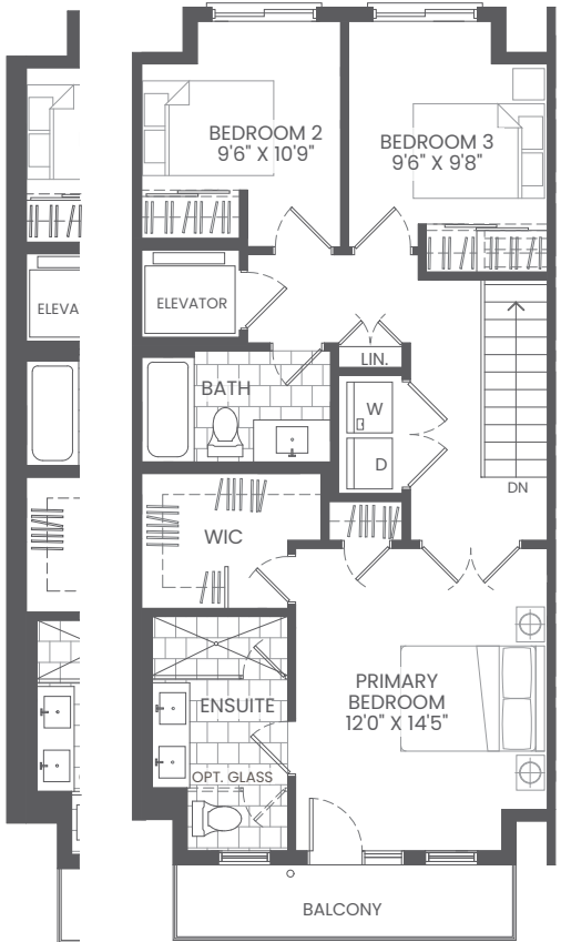
PART. END UPPER FLOOR STANDARD BLKB & C UPPER FLOOR STANDARD INTERIOR BLK B & C
